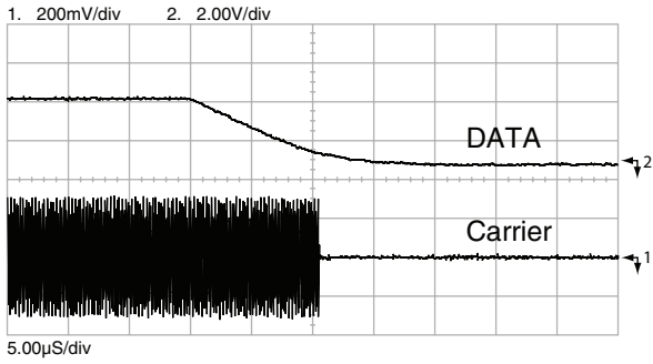
Figure 17: TX Turn-Off Time
