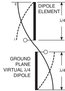
Figure 34: Dipole Antenna
