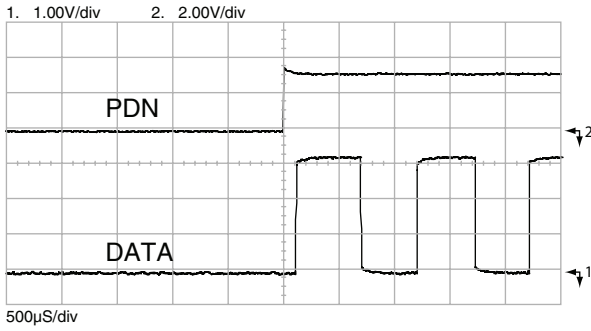
Figure 12: RX Turn-On Time from PDN
