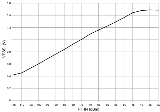
Figure 8: RSSI Curve
