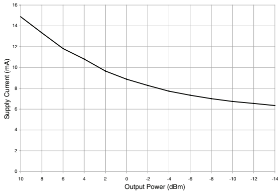
Figure 7: Output Power vs. Current Consumption
