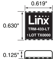
Figure 1: Package Dimensions
