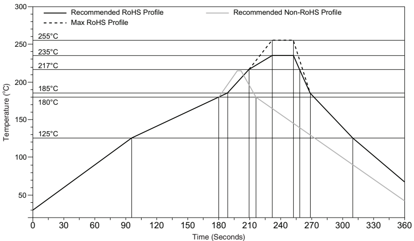
Figure 31: Maximum Reflow Profile
