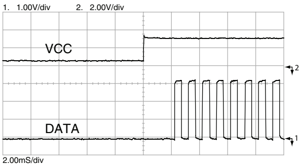
Figure 11: TX to RX Change Time
