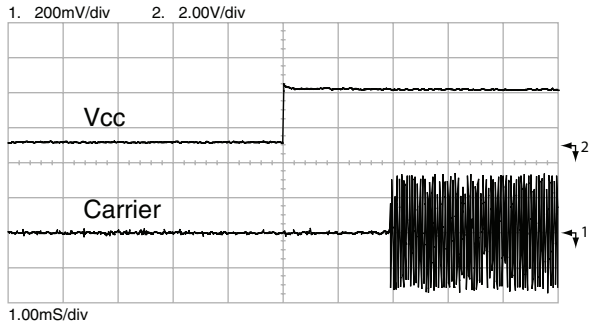
Figure 16: TX Turn-On Time from V_{CC}
