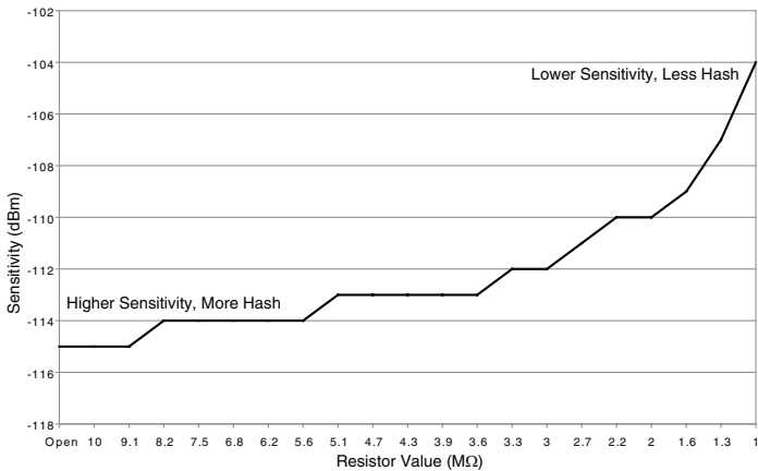
Figure 23: Sensitivity Degradation vs. Squelch Resistor
