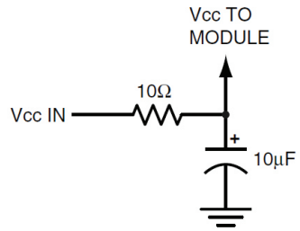
Figure 22: Supply Filter
