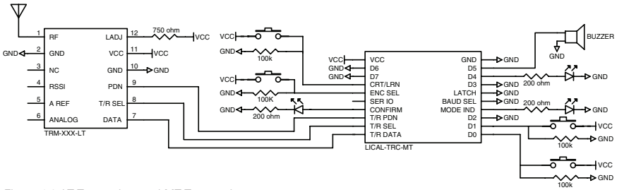
Figure 24: LT Transceiver and MT Transcoder
