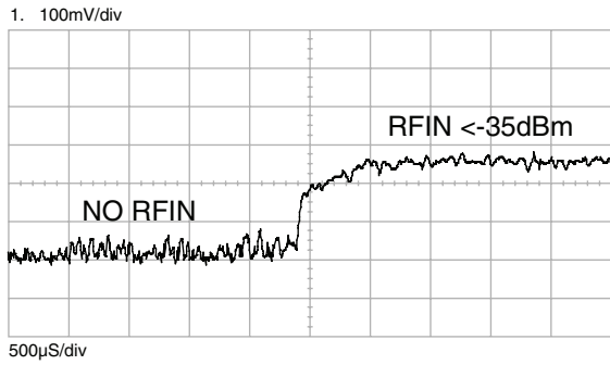
Figure 13: RSSI Response Time
