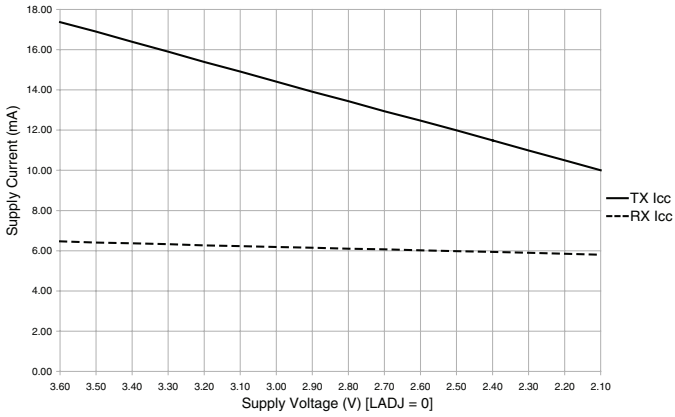
Figure 9: Current Consumption vs. Supply
