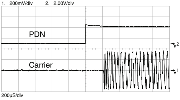
Figure 15: TX Turn-On Time from PDN
