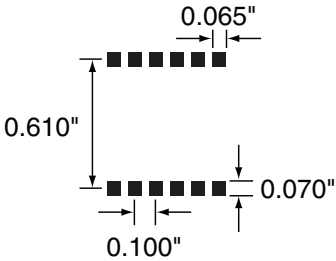
Figure 28: Recommended PCB Layout
