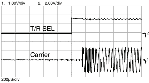
Figure 10: RX to TX Change Time
