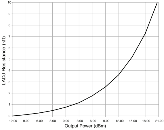
Figure 6: Output Power vs. LADJ Resistance
