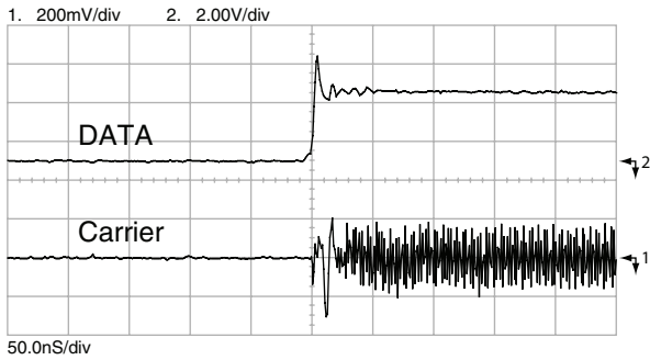
Figure 14: TX Modulation Delay
