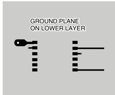
Figure 25: Suggested PCB Layout
