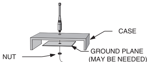
Figure 35: Remote Ground Plane
