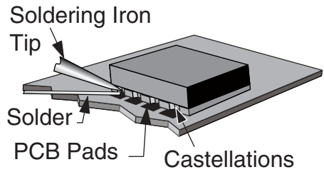
Figure 29: Soldering Technique
