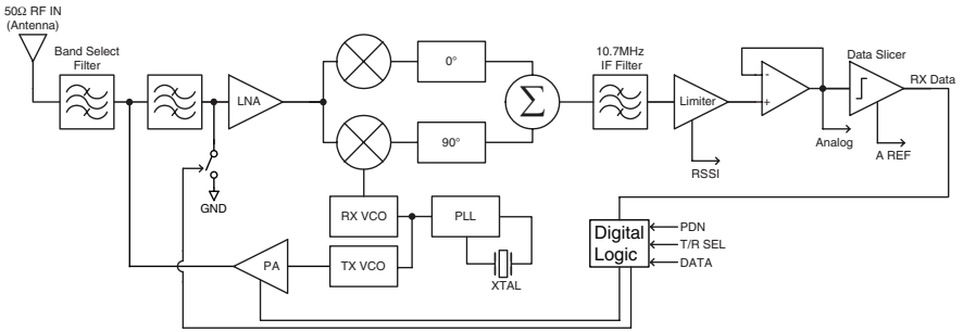
Figure 20: LT Series Transceiver Block Diagram
