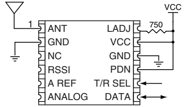
Figure 5: Test / Basic Application Circuit
