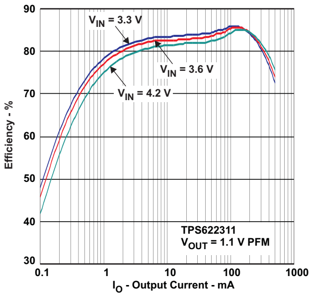
Figure 11. Comparison Efficiency vs IOUT – TPS622311
