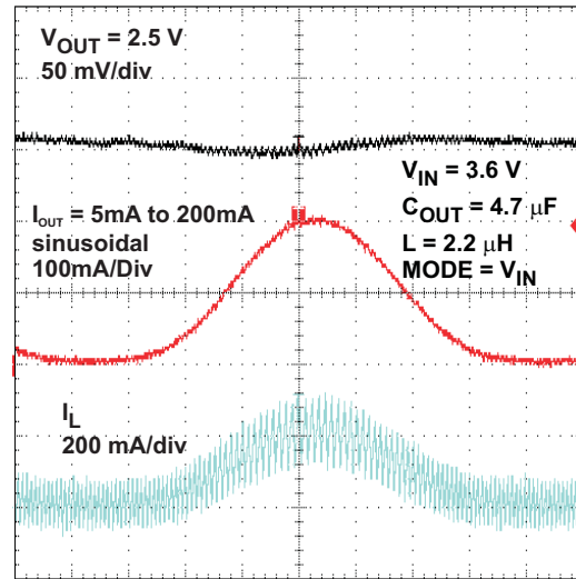
Figure 42. AC – Load Regulation Performance 2.5V V_{OUT} PWM Mode
