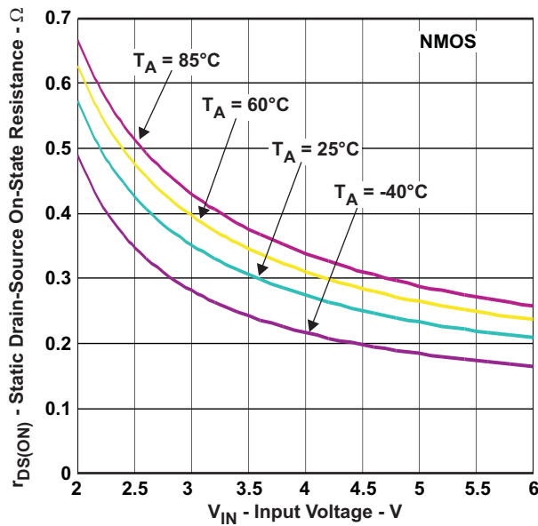
Figure 33. NMOS R_{DS(ON)} vs Supply Voltage V_{IN} and Ambient Temperature T_A
