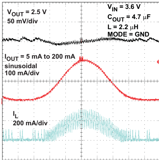
Figure 41. AC – Load Regulation Performance 2.5V V_{OUT} PFM Mode
