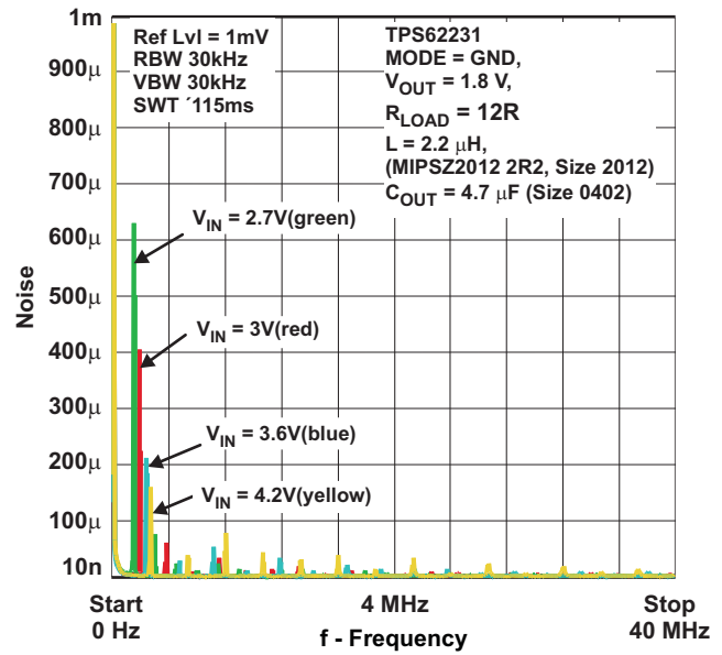
Figure 50. Spurious Output Noise, 12R Load, TPS62231
