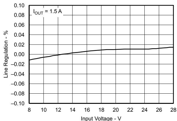
Figure 44. TPS54336 DRC Line Regulation
