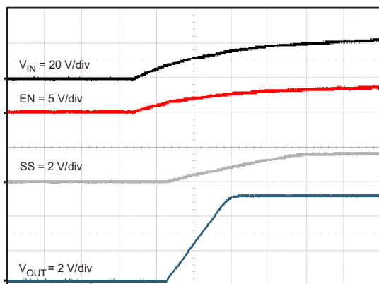
Figure 51. TPS54336 Start Up Relative to VIN
