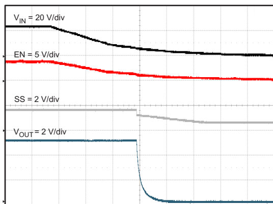
Figure 53. TPS54336 Shut Down Relative to VIN
