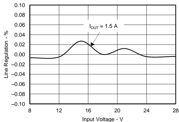
Figure 43. TPS54336 DDA Line Regulation
