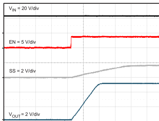
Figure 52. TPS54336 Start-up Relative to Enable
