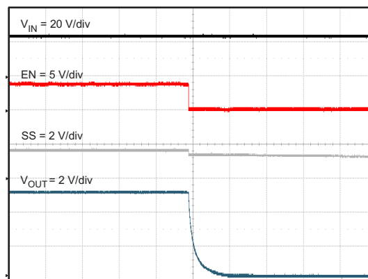
Figure 54. TPS54336 Shut Down Relative to EN
