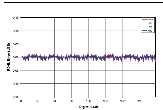
Figure 5. DNL vs. TAP POSITION (Rheostat Mode)
