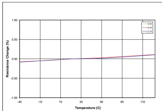
Figure 6. End to End resistance change vs Temperature
