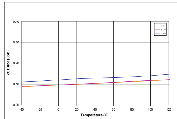
Figure 7. Zero Scale Error vs Temperature
