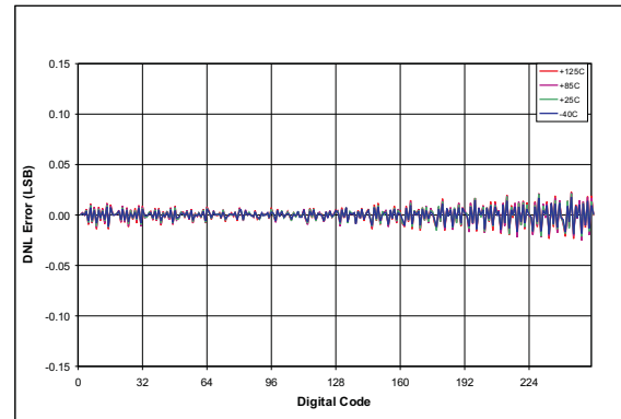
Figure 3. DNL vs TAP POSITION (Potentiometer Mode)
