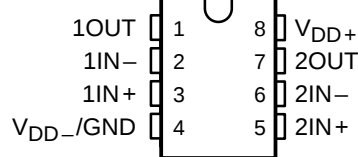
TLC2252M, TLC2252AM . . . JG PACKAGE (TOP VIEW)
