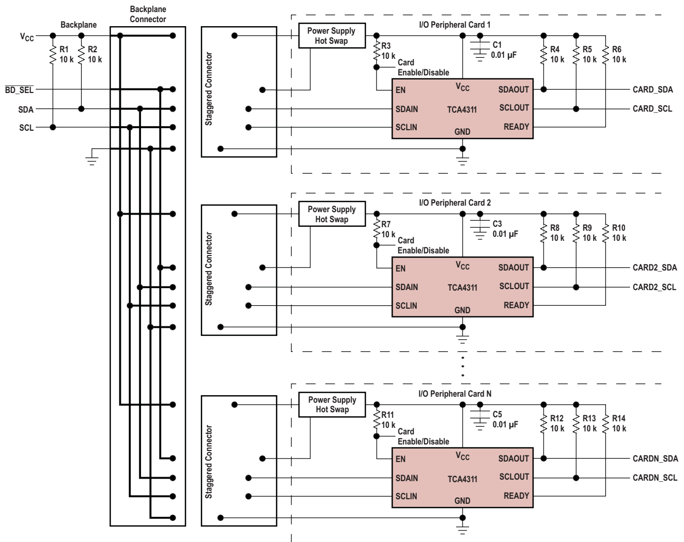
Figure 10. Inserting Multiple I/O Cards into a Live Backplane Using the TCA4311A in a CompactPCI System
