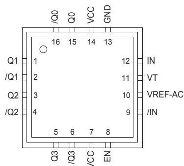
16-Pin QFN
