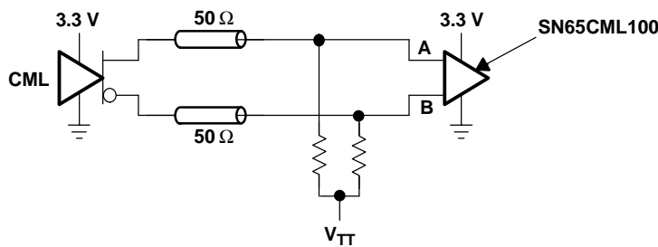
Figure 25. Current-Mode Logic (CML)
