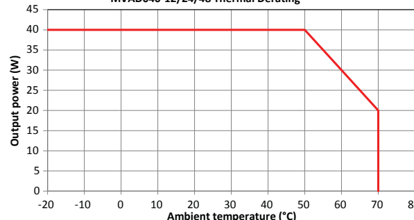
MVAD040-12/24/48 Thermal Derating
