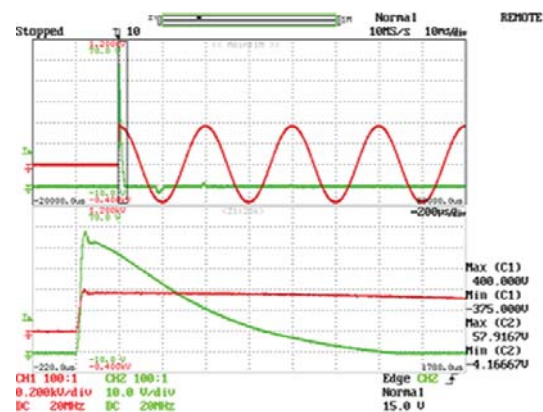
Inrush waveform
