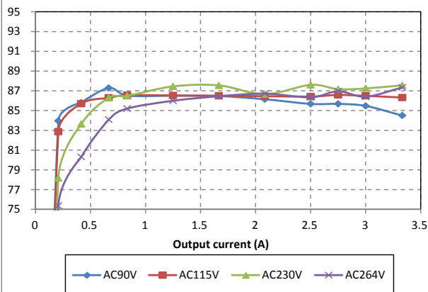
MVAD040-12 Efficiency (%)
