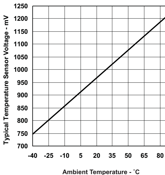
Figure 17. Typical Temperature Sensor Voltage
