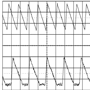
Figure 40. CCM and DCM Operating Modes V_{IN} = 12V, V_O = 3.3V, I_O = 2A/0.26A \ 2 \mu sec/div
