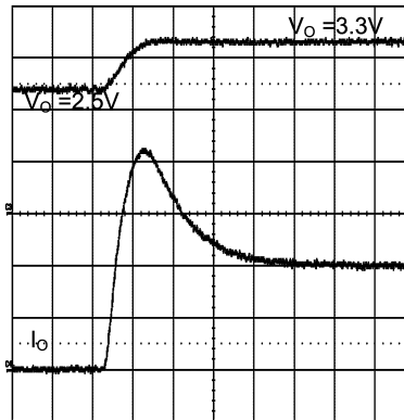
Figure 42. Pre-Biased Startup
