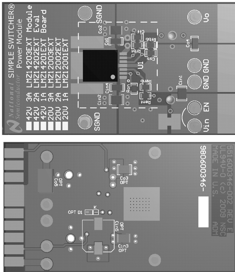
Figure 43. PCB Layout Example
