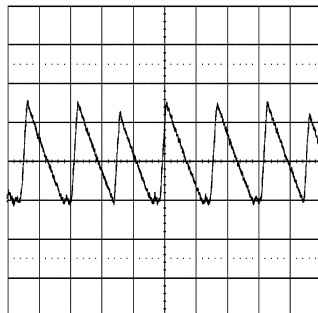
Figure 41. Transition Mode Operation V_{IN} = 12V, V_O = 3.3V, I_O = 0.29A \ 2 \mu sec/div
