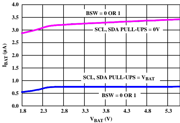
FIGURE 1. I_{BAT} vs V_{BAT} , SBIB = 0
