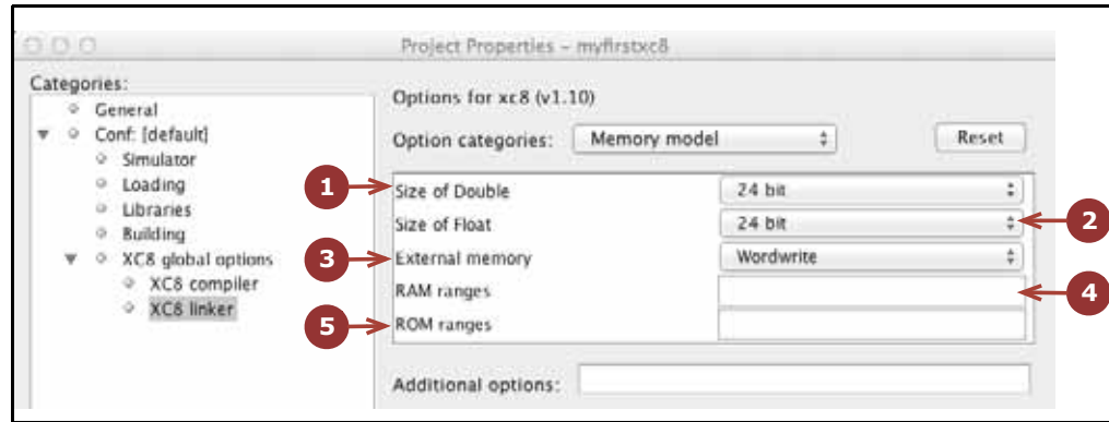
FIGURE 4-12: MEMORY MODEL OPTIONS
