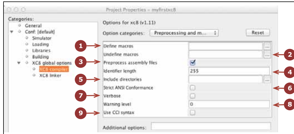
FIGURE 4-9: PREPROCESSING AND MESSAGES OPTIONS
