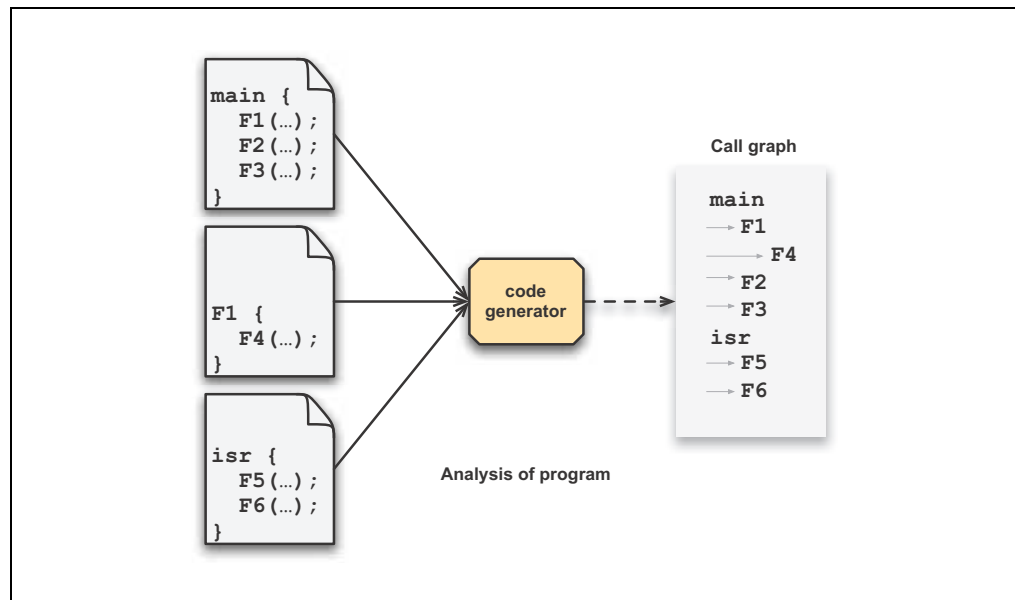
FIGURE 5-2: FORMATION OF CALL GRAPH
