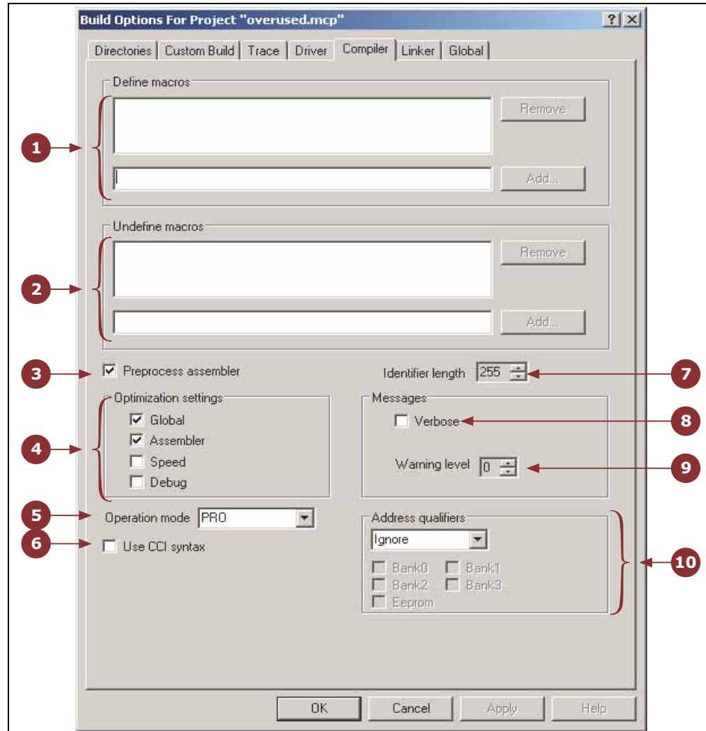
FIGURE 4-6: THE COMPILER TAB
