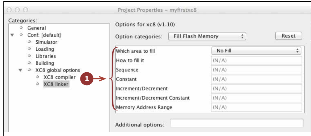
FIGURE 4-13: FILL FLASH MEMORY OPTIONS
