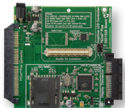
Graphics LCD Controller PICTail Plus SSD1926 Board (AC164127-5)
