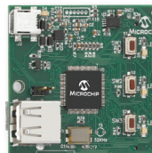
dsPIC33E USB Starter Kit (DM330012)
