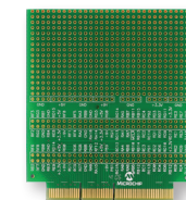
Prototype PICTail Plus Daughter Board (AC164126)
