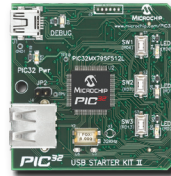
PIC32 USB Starter Kit II (DM320003-2)
