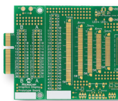
Graphics Display Prototype Board (AC164139)
