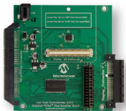
Low-Cost Controllerless (LCC) Graphics PICTail Plus Daughter Board (AC164144)
