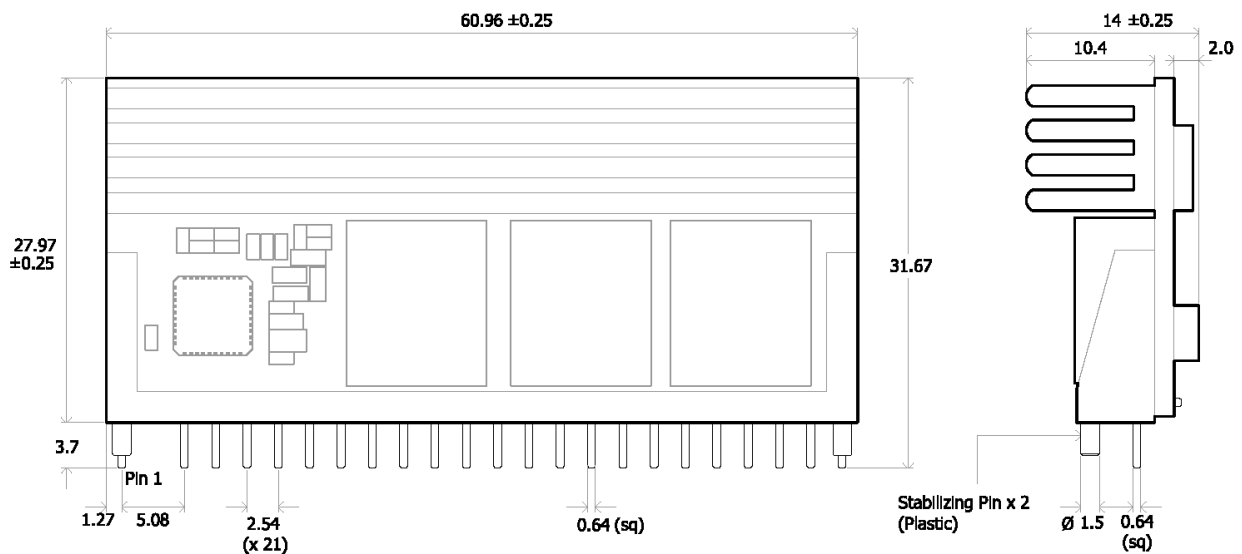
Figure 51. Mechanical Drawing
