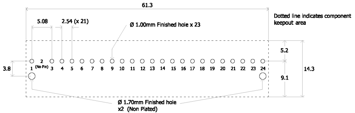
Figure 52. Recommended Footprint – Top View
