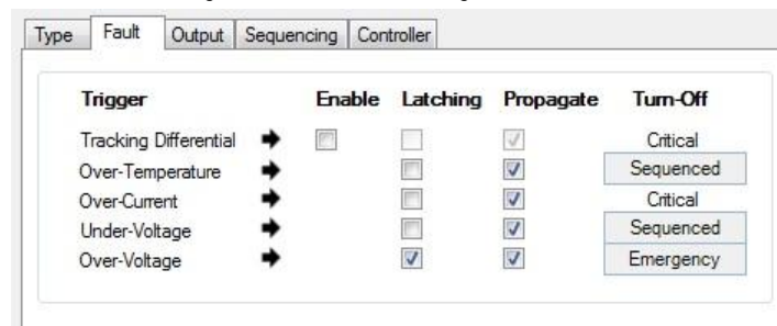
Figure 26. dPOL Fault Management Window
