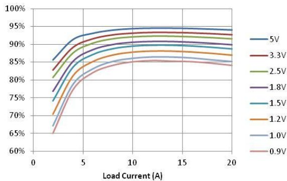
Figure 5. Efficiency vs. Load, V_{in} = 8\text{ V} , F_{sw} = 500\text{ KHz}
