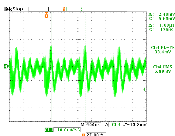
Figure 46. Input Voltage Noise with Interleave
