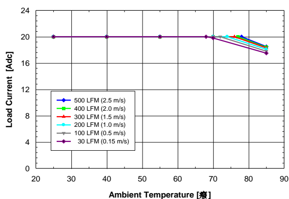
Figure 1. Available output current vs. ambient air temperature and airflow rates for converter DP8120G mounted horizontally with air flowing from input to output, MOSFET temperature \leq 120^{\circ}\text{C} , V_{in} = 8\text{ V} , V_{out} = 5\text{ V} , and F_{sw} = 500\text{KHz}
