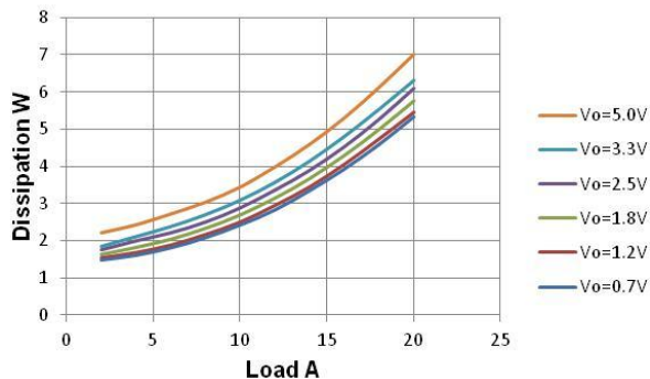
Figure 9. Dissipation vs Load, V_{in} = 12\text{ V} , F_{sw} = 500\text{ KHz}
