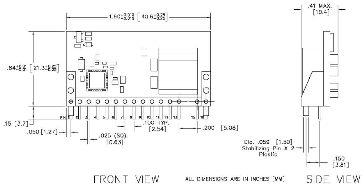
Figure 58. Mechanical Drawing
