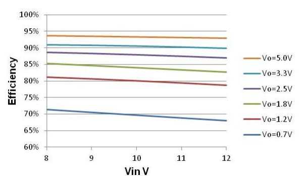
Figure 10. Efficiency vs Vin, I_{out} = 20\text{ A} , F_{sw} = 1\text{ MHz}
