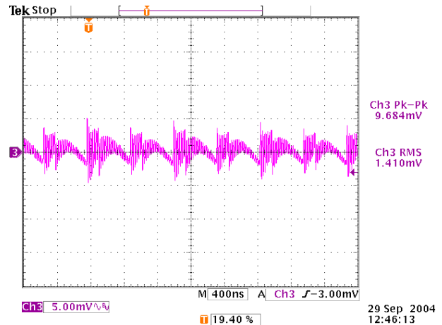
Figure 48. Output Voltage Noise, Full Load, 180° Interleave
