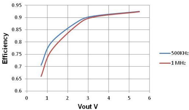
Figure 5. Efficiency vs. Output Voltage, I_{out}=10\text{A} , F_{sw}=500\text{kHz} and F_{sw}=1\text{MHz}
