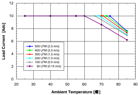
Figure 1. Available output current vs. ambient air temperature and airflow rates for converter DP8110G mounted horizontally with air flowing from input to output, MOSFET temperature \leq 120\text{ }^{\circ}\text{C} , V_{in} = 12\text{ V} , V_{out} = 5\text{ V} , and F_{sw} = 500\text{KHz}
