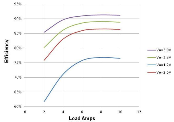
Figure 4 Efficiency vs. Load. V_{in}=12\text{V} , F_{sw}=1\text{MHz}
