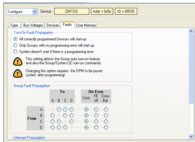
Figure 33. DPM Configure Faults Window
