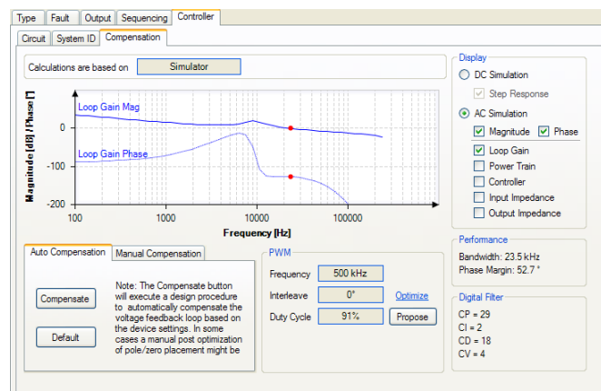
Figure 40. PWM Controller Window
