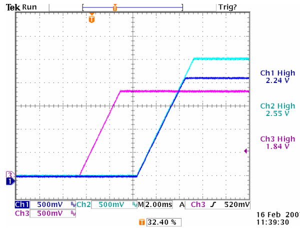
Figure 23 Two outputs delayed 5ms. All slew rates at 0.5V/ms.
