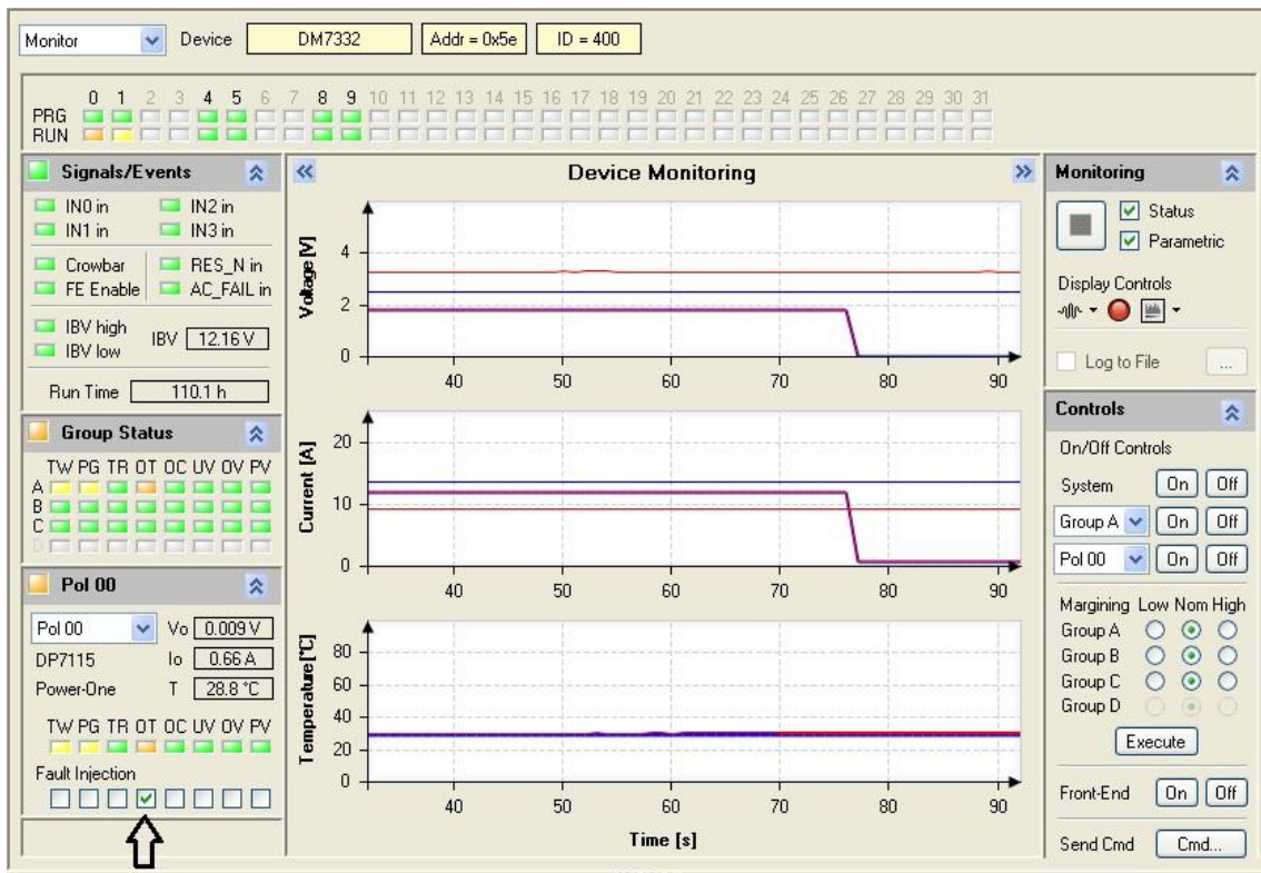
Figure 52. Example Overtemp Fault Injection in the GUI
