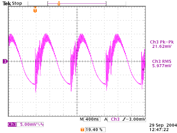
Figure 44. Output Voltage Noise, Full Load, No Interleave
