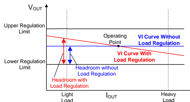
Figure 12. Optimal Voltage Positioning Concept
