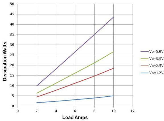
Figure 8. Dissipation vs Load. Vin=12V, Fsw=500kHz
