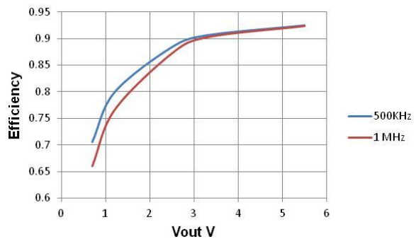
Figure 6 Efficiency vs Vout, V_{in}=12 , Load=10A
