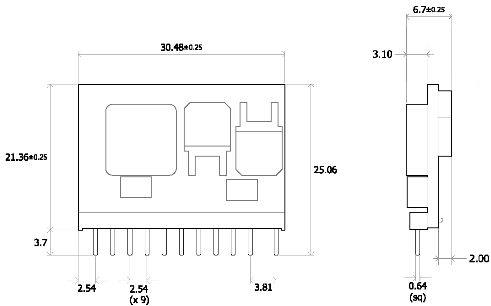
Figure 55 - Mechanical Drawing
