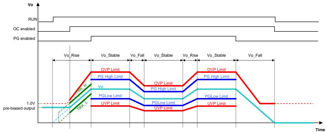
Figure 29. Protection Enable Conditions
