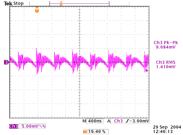
Figure 45. Output Voltage Noise, Full Load, 180° Interleave
