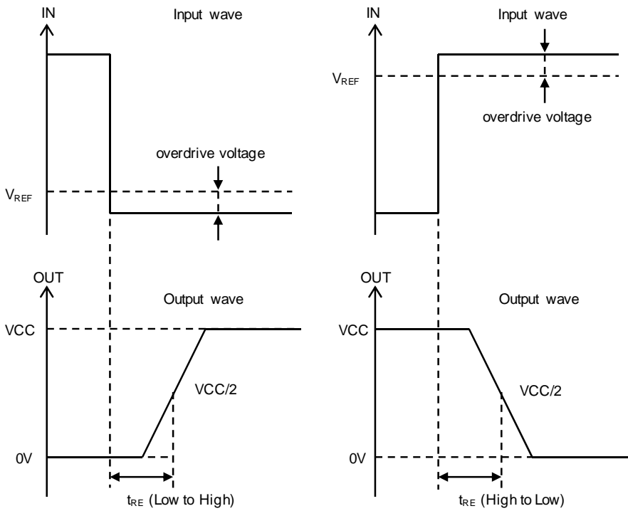
Figure 113. Response Time
