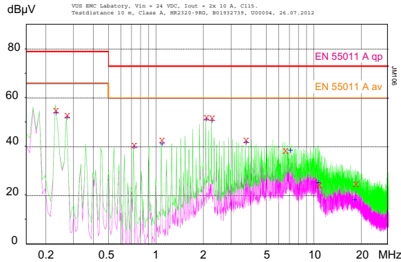
Fig. 16a Typ. conducted emissions (peak/quasipeak and average) at the input according to EN 55011/22, measured at V_i = 24 V and I_{o\text{ nom}} (HR2320-9RG).
