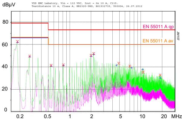
Fig. 16b Typ. conducted emissions (peak/quasipeak and average) at the input according to EN 55011/22, measured at V_i = 110 V and I_{o\text{ nom}} (HR2320-9RG).
