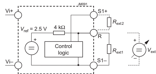
Fig. 13 Output voltage adjustment
