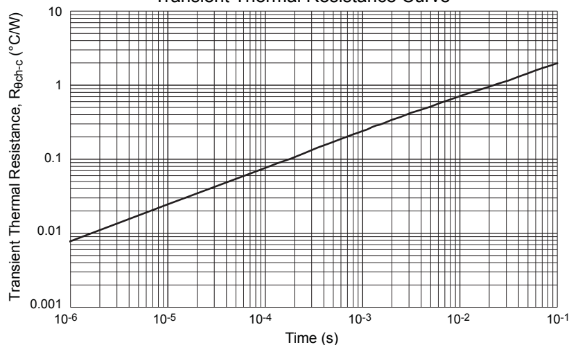
Transient Thermal Resistance Curve
