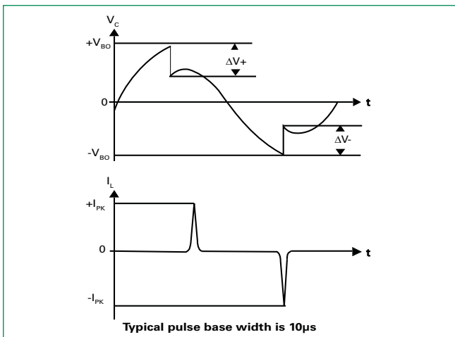
Figure 8: Test Circuit Waveform
