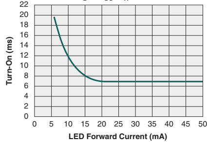
Typical Turn-On vs. LED Forward Current ( I_L=1\text{A}_{\text{DC}} , T_A=25^\circ\text{C} )
