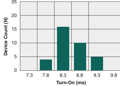
Typical Turn-On Time (N=35, I_F=20\text{mA} , I_L=1\text{A}_{\text{DC}} , T_A=25^\circ\text{C} )
