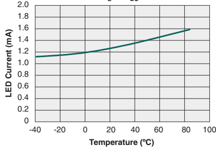
Typical I_F for Switch Operation vs. Temperature ( I_L=1\text{A}_{\text{DC}} )
