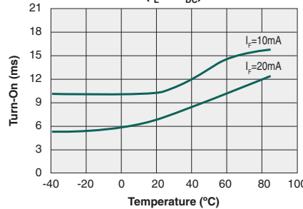
Typical Turn-On vs. Temperature ( I_L=1\text{A}_{\text{DC}} )
