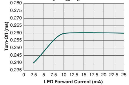
Typical Turn-Off vs. LED Forward Current ( I_L=1\text{A}_{\text{DC}} , T_A=25^\circ\text{C} )
