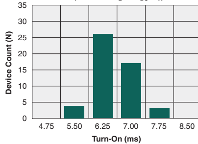
Typical Turn-On Time (N=50, I_F=20\text{mA} , I_L=1\text{A}_{DC} , T_A=25^\circ\text{C} )
