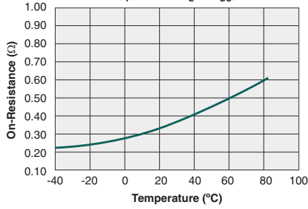
Typical On-Resistance vs. Temperature ( I_F=10\text{mA} , I_L=1A_{DC} )
