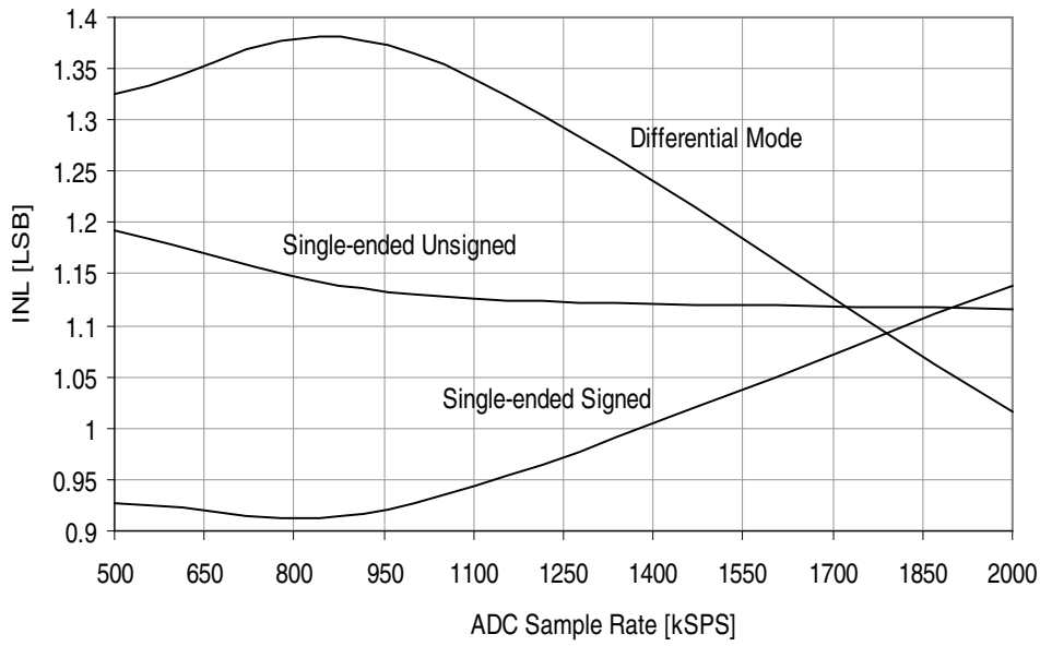
Figure 37-292. INL error vs. sample rate. T = 25°C, V CC = 3.6V, V REF = 3.0V external.
