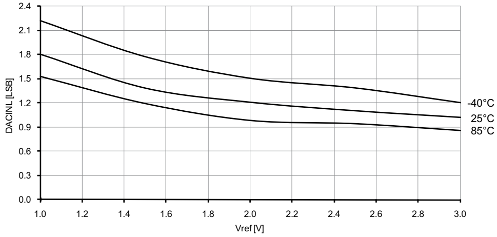
Figure 37-219. DAC INL error vs. V_{REF} . V_{CC} = 3.6V .
