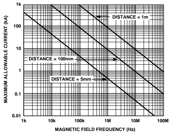
Figure 44. Maximum Allowable Current for Various Current-to-ADuM347x Spacings
