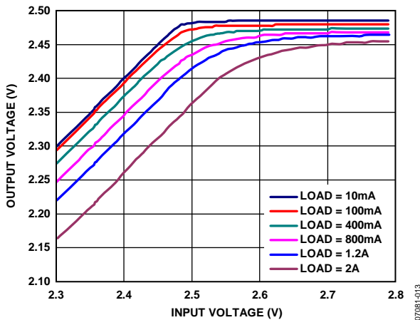
Figure 13. Output Voltage vs. Input Voltage (in Dropout), V_{OUT} = 2.5\text{ V}
