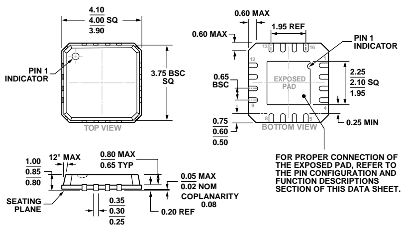
Figure 49. 16-Lead Lead Frame Chip Scale Package [LFCSP_VQ] 4 mm × 4 mm Body, Very Thin Quad (CP-16-4) Dimensions shown in millimeters
