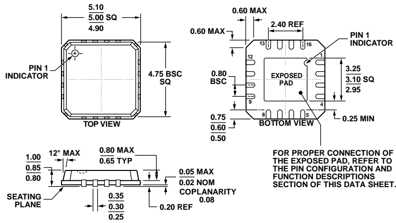
Figure 27. 16-Lead Lead Frame Chip Scale Package [LFCSP_VQ] 5 mm × 5 mm Body, Very Thin Quad CP-16-6 Dimensions shown in millimeters
