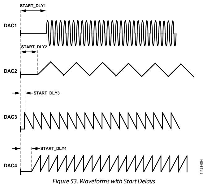
Figure 53. Waveforms with Start Delays
