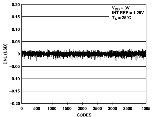
Figure 24. DNL AD5628-1
