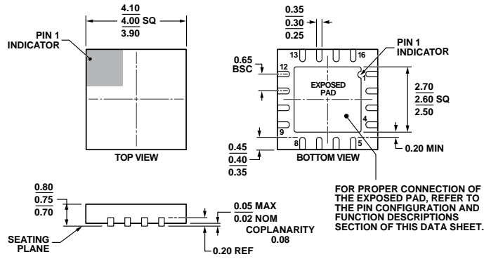
Figure 64. 16-Lead Lead Frame Chip Scale Package [LFCSP_WQ] 4 mm × 4 mm Body, Very Very Thin Quad (CP-16-17)
