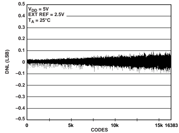
Figure 17. DNL AD5648-2
