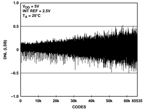
Figure 16. DNL AD5668-2/AD5668-3
