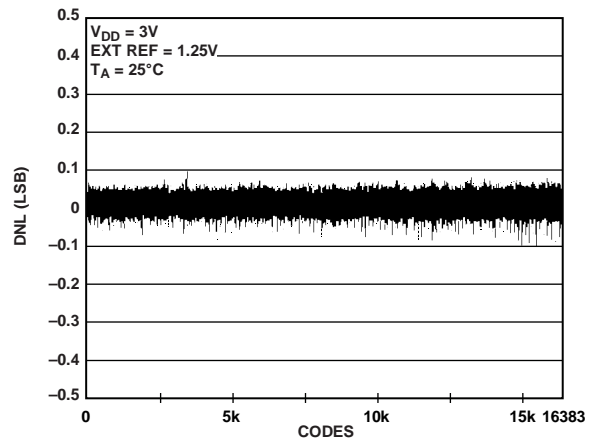
Figure 23. DNL AD5648-1
