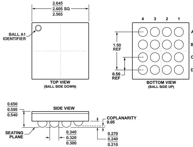
Figure 65. 16-Ball Wafer Level Chip Scale Package [WLCSP] (CB-16-16)
