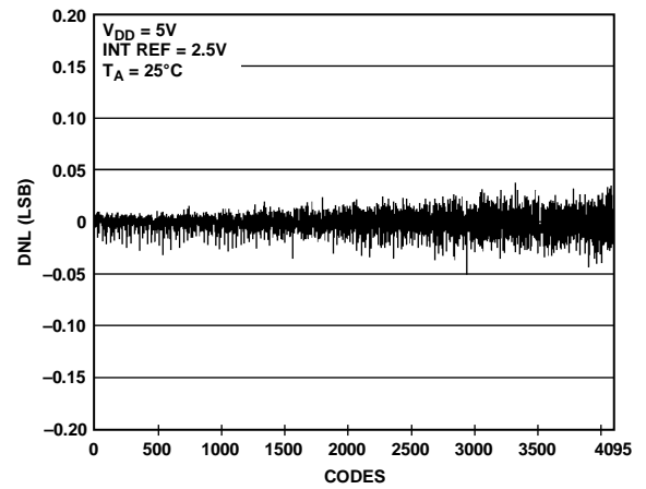
Figure 18. DNL AD5628-2
