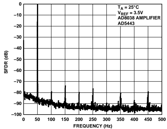
Figure 35. Wideband SFDR f_{OUT} = 50\text{ kHz} , Update = 1 MHz
