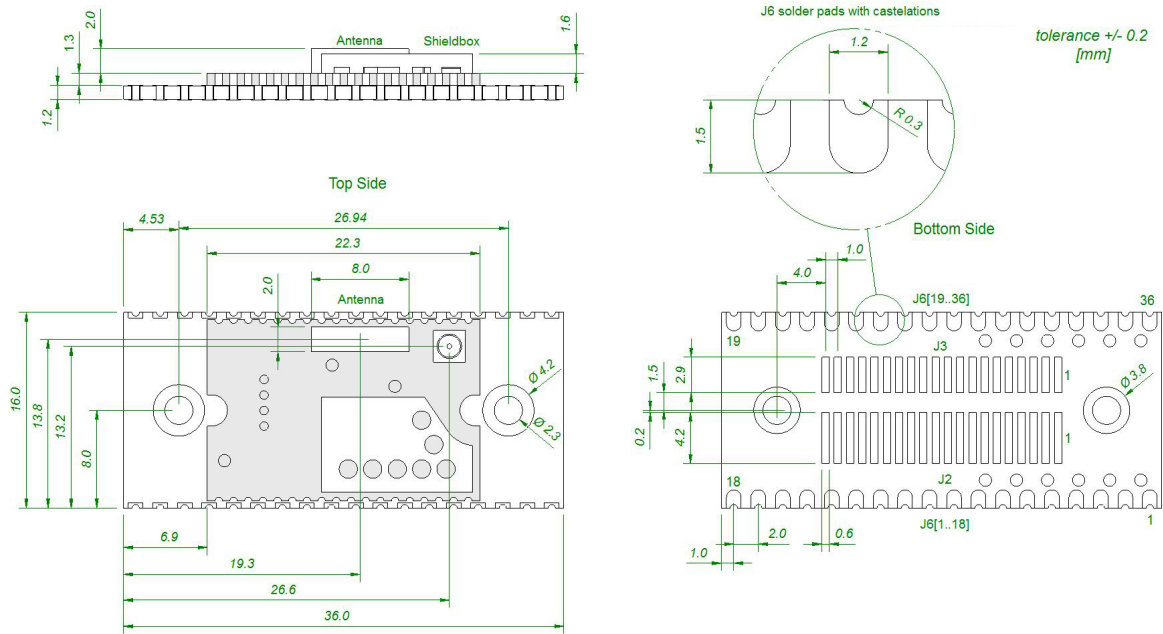
Figure 13: cB-OLS426 dimensions.
